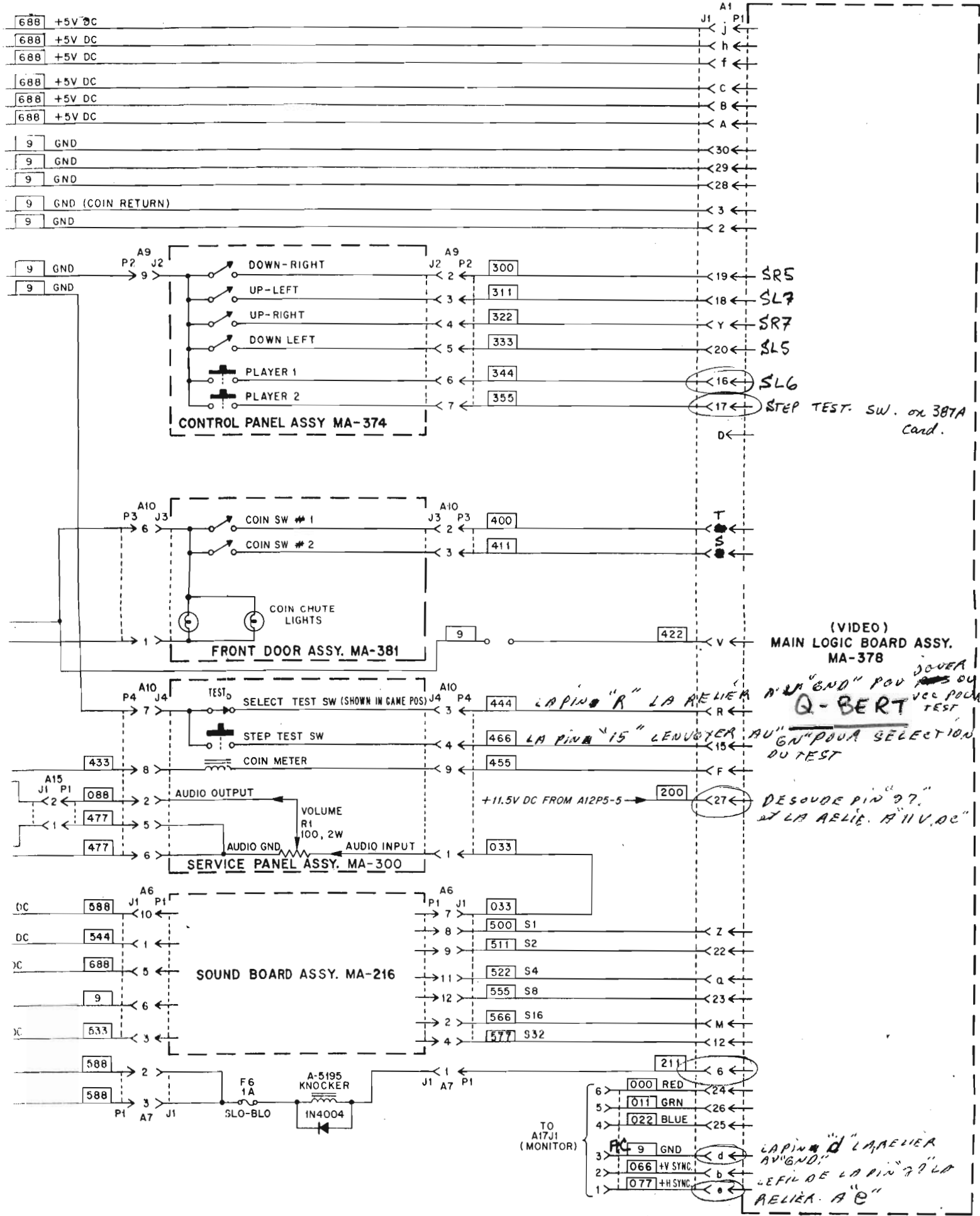
PRIMARY POWER/INTERCONNECTION DIAGRAM
