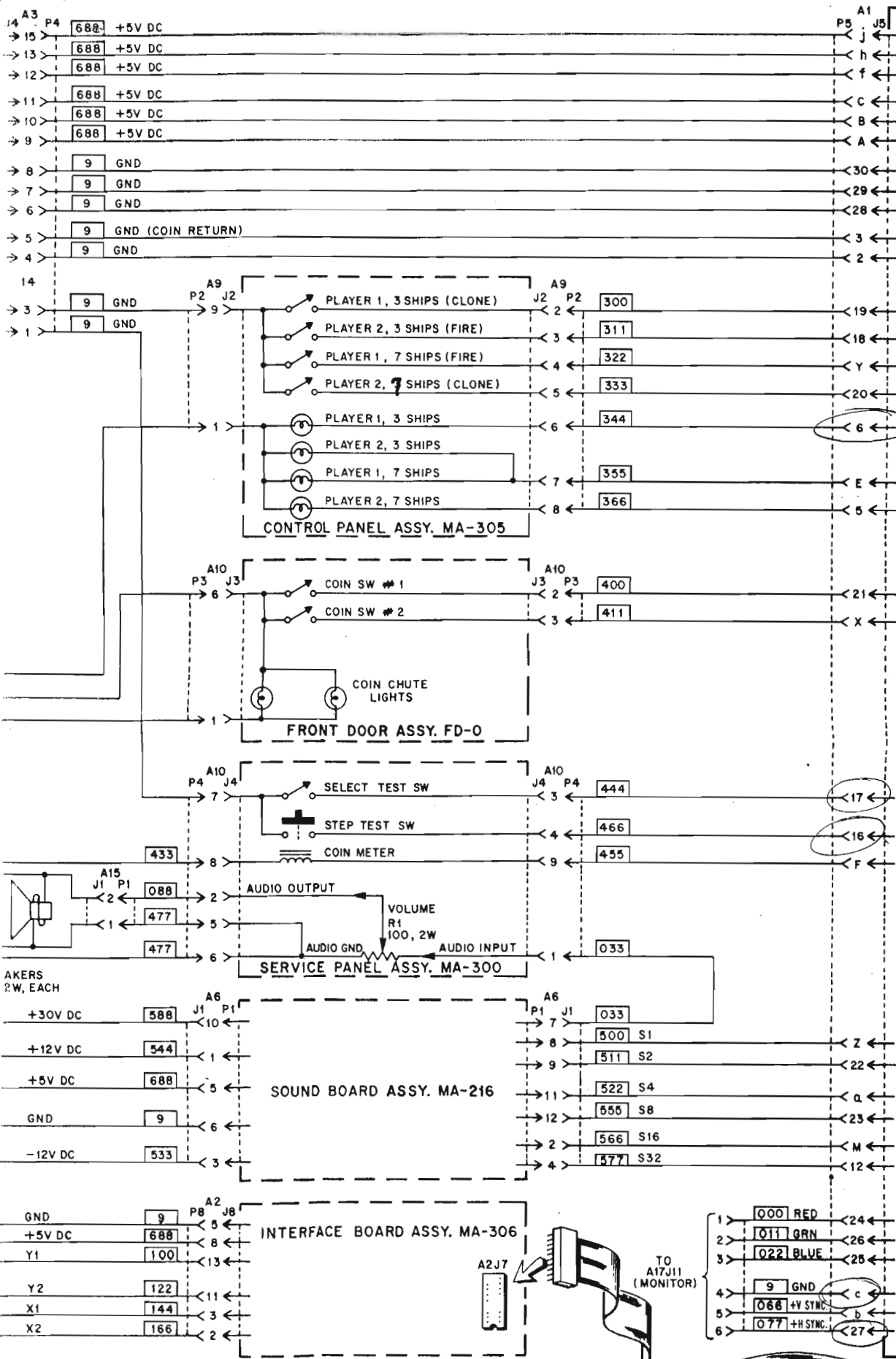
PRIMARY POWER/INTERCONNECTION DIAGRAM
