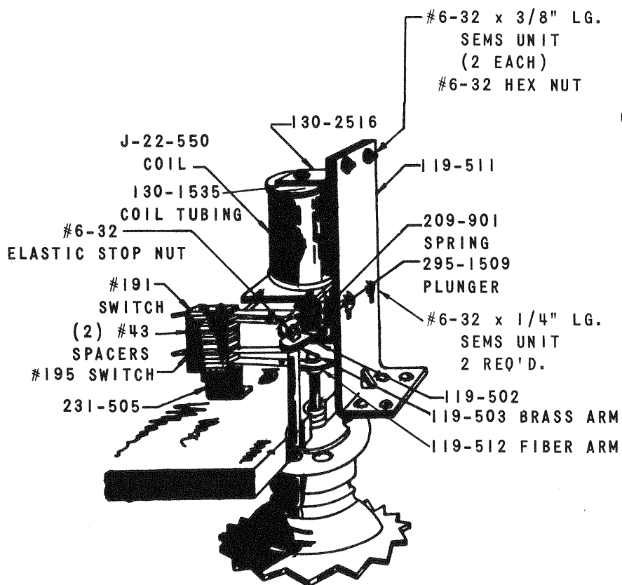
THUMPER BUMPER COMPLETE ASSEMBLY
