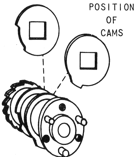
143-2511 HUB, CAM AND RATCHET ASSEMBLY
