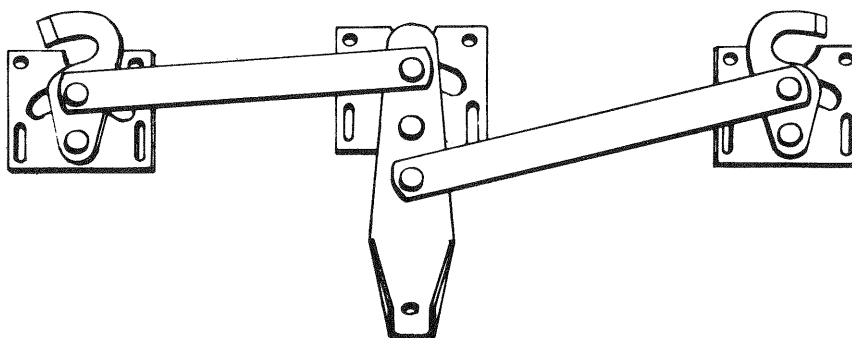
295-2520 FRONT MOLDING LOCK ASSEMBLY
