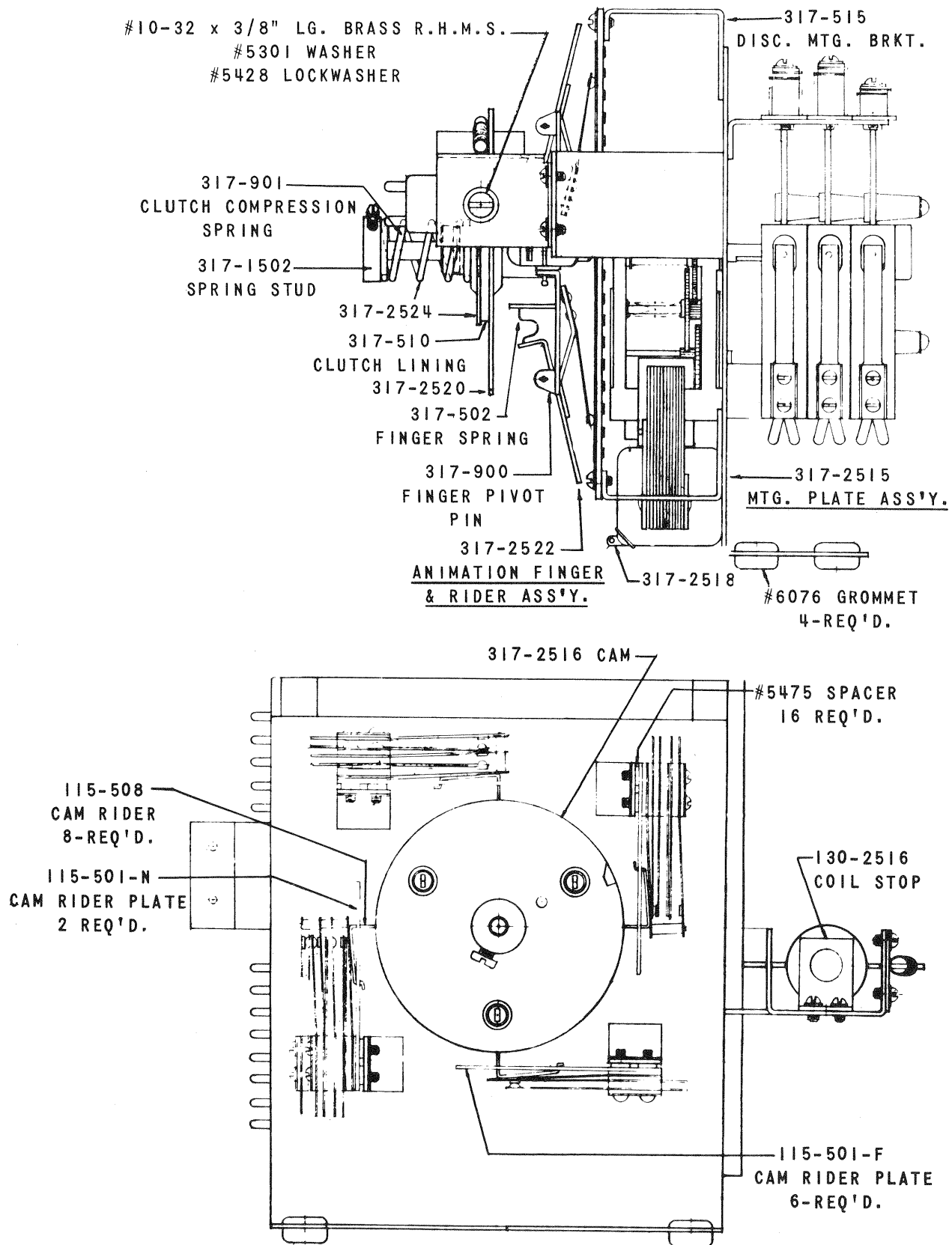
317-2514 BASE ANIMATION ASSEMBLY
