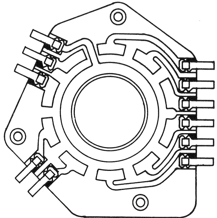
151-2540 CONTACT PLATE ASSEMBLY (WIPER FINGER ASSEMBLY FOR ABOVE 151-2542)
