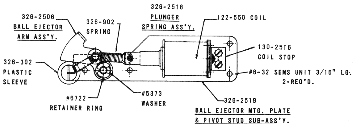
326-2520 BALL EJECTOR ASSEMBLY
