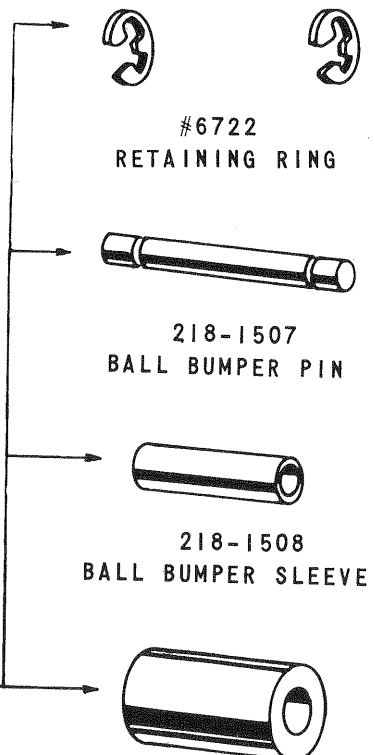
218-2517 BALL BUMPER RUBBER SLEEVE
