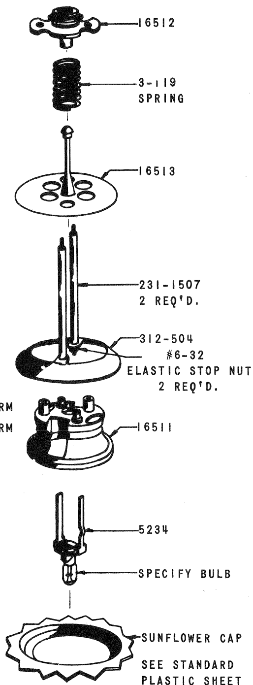
THUMPER BUMPER BREAKDOWN
