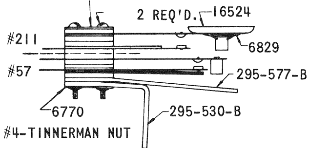
TARGET SWITCH
