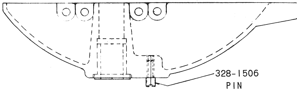
328-2534 TURRET CASTING ASSEMBLY (TEXAS RANGER)
