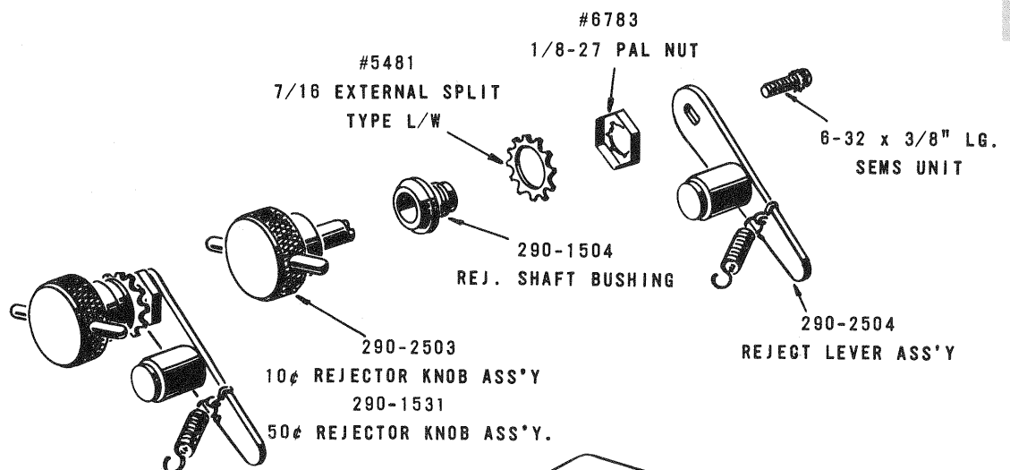
FRONT REJECTOR ASS'Y
