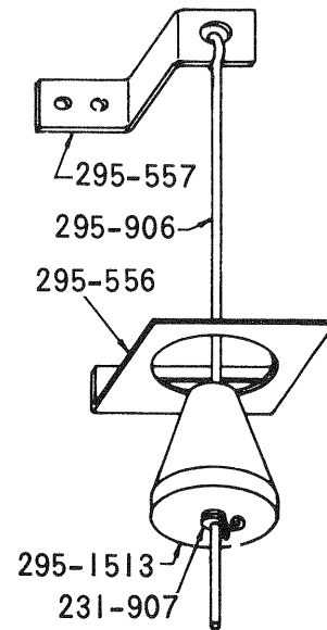
TILT PLUMB SWITCH ASSEMBLY
