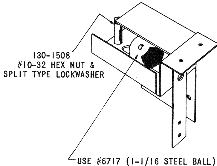
ELEVATOR TILT ASSEMBLY
