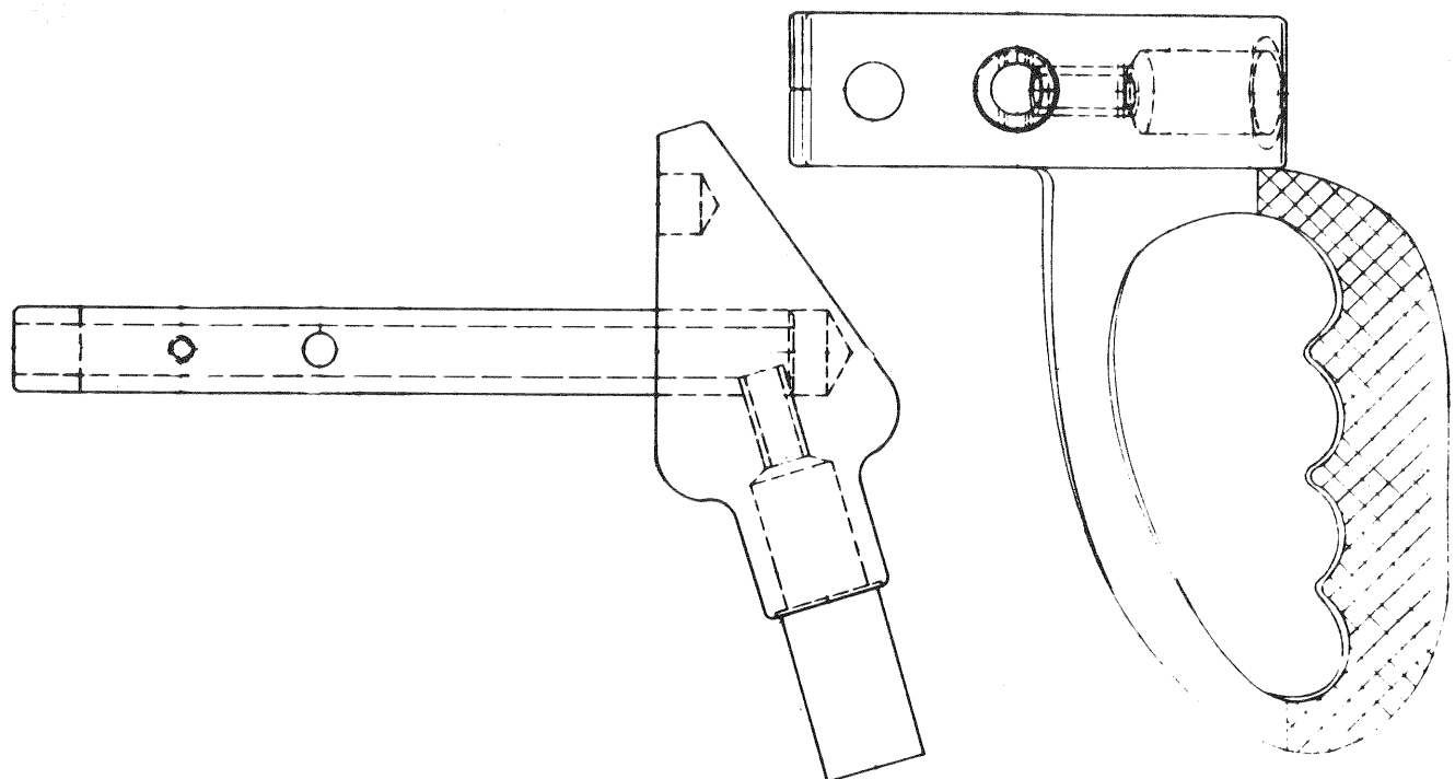
328-2522 L or R R-HANDLE AND SHAFT ASSEMBLY (TEXAS RANGER)
