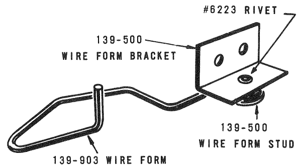
242-2505 PUCK ROLL OVER ASS'Y.
